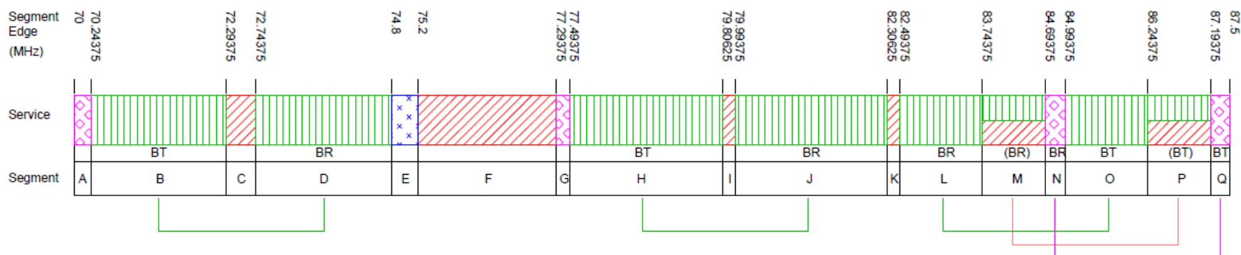
Figure 1: Illustration of VHF Mid-Band spectrum arrangements
